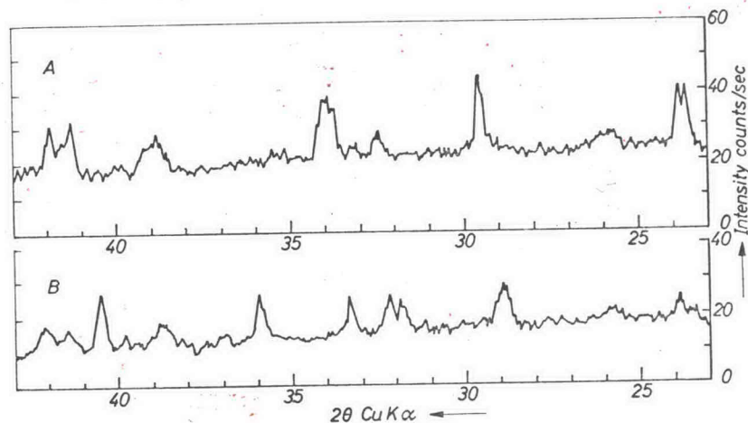
Fig. 3. A. \text{KNO}_3 II at room pressure. \text{CuK}\alpha radiation. Note the partially resolved 111 and 021 peaks at 23+ degrees, that were completely unresolved in Fig. 2 A. Bridgman anvil device with beryllium pellets; B. \text{KNO}_3 IV at 6.6 kbar (nominal), \text{CuK}\alpha radiation. Note the completely resolved 030 and 400 peaks at 32 degrees that were only partially resolved in Fig. 2 B. Bridgman anvil device with beryllium pellet. Attenuation 4-1-8. Pellet 5.0 mm diam.
