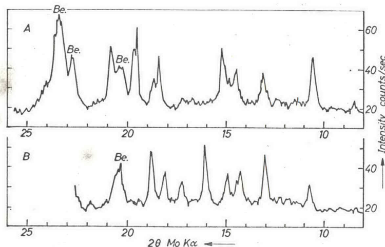
Fig. 2. A. \text{KNO}_3 II at room pressure, \text{MoK}\alpha radiation. The large peak between ten and eleven degrees is actually a doublet, 111 and 021, not resolved. Supported beryllium cylinder; B. \text{KNO}_3 IV at 3.7 kb, \text{MoK}\alpha radiation. Note the two peaks only slightly resolved at about 14.3 degrees. These are 030 and 400 of the high-pressure form. Supported beryllium cylinder. Attenuation 4-1-8. Pellet 4.6 \times 1.0 mm diam.
